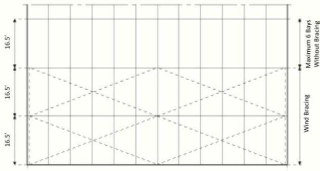
98' Structure Top Elevation
